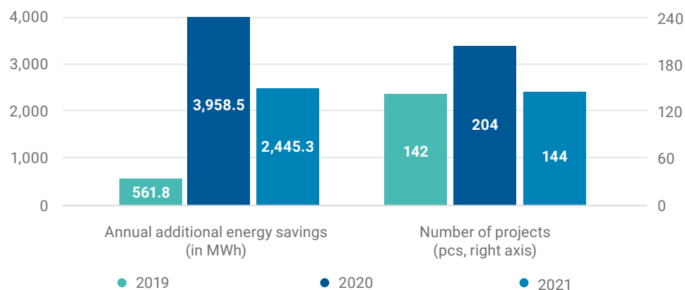
Figure 19: Energy Savings due to the Hungarian Rural Development Program Focus Area 5B.
